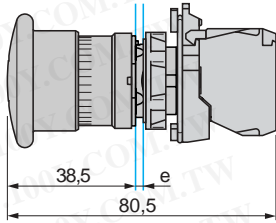
Emergency stop mushroom head pushbuttons XB5-AT845
