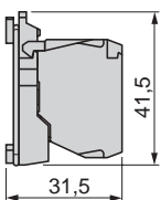
Bodies for pushbuttons, screw clamp terminal connections ZB5-AZ10, AZ141
