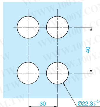
Support panel cut-out
