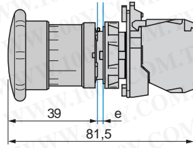
Emergency stop mushroom head pushbuttons XB5-AT845
