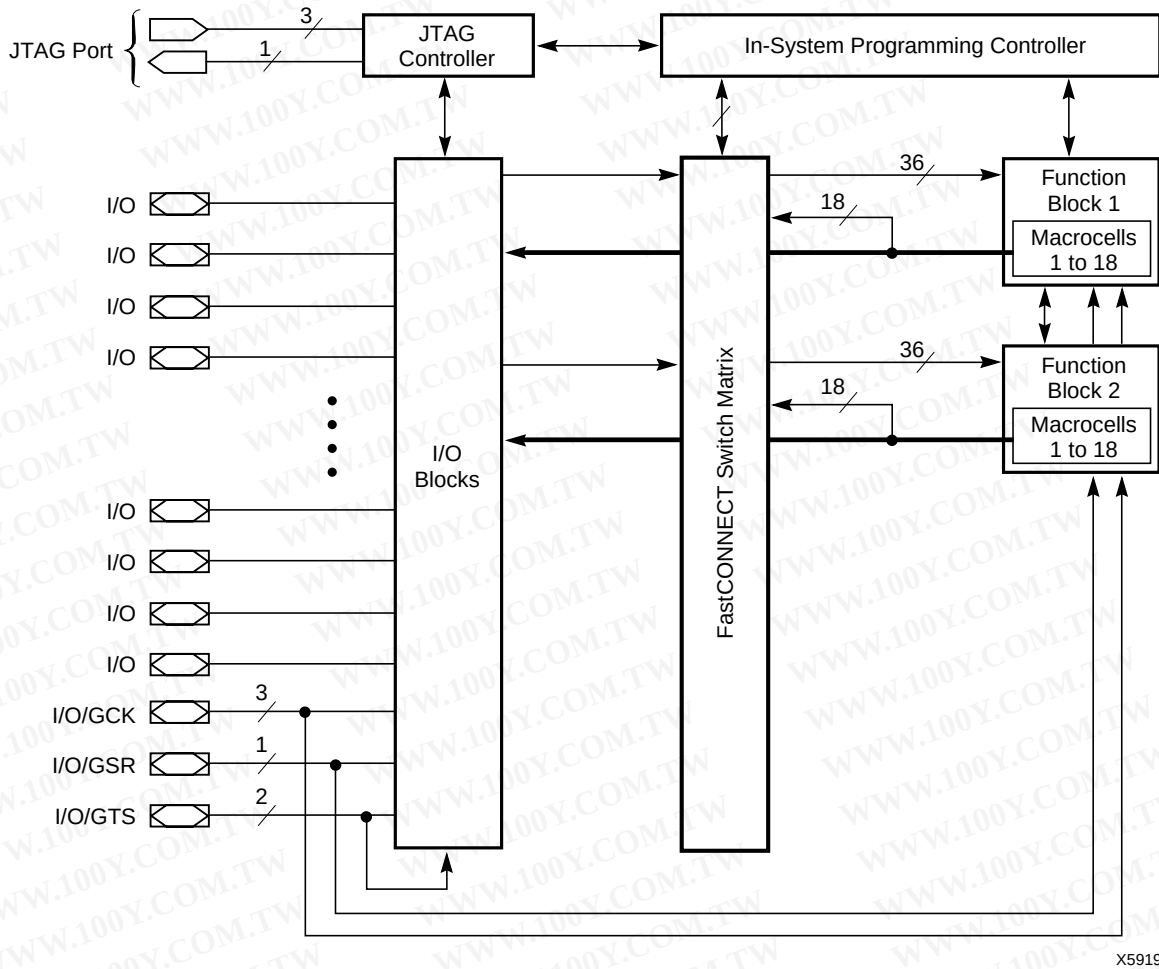
Figure 2: XC9536 Architecture
