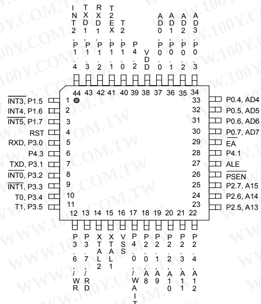
44-Pin QFP
