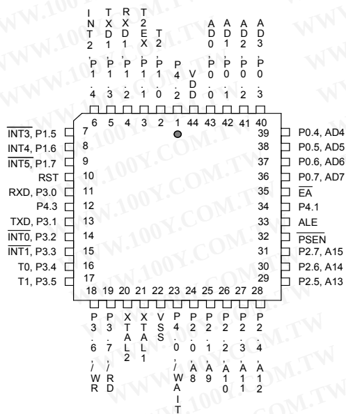
44-Pin PLCC
