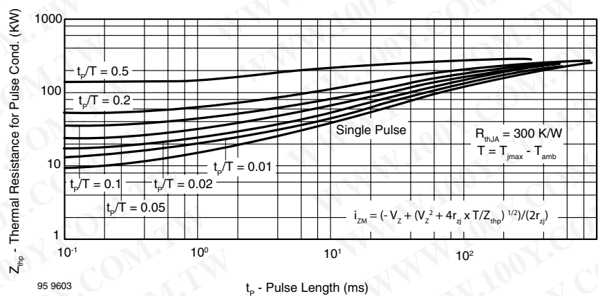
Figure 10. Thermal Response
