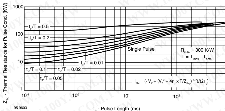
Figure 13. Thermal Response
