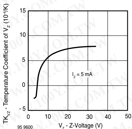
Figure 3. Temperature Coefficient of V_Z vs. Z-Voltage
