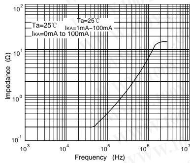
Fig 5 Dynamic Impedance Vs Frequency
