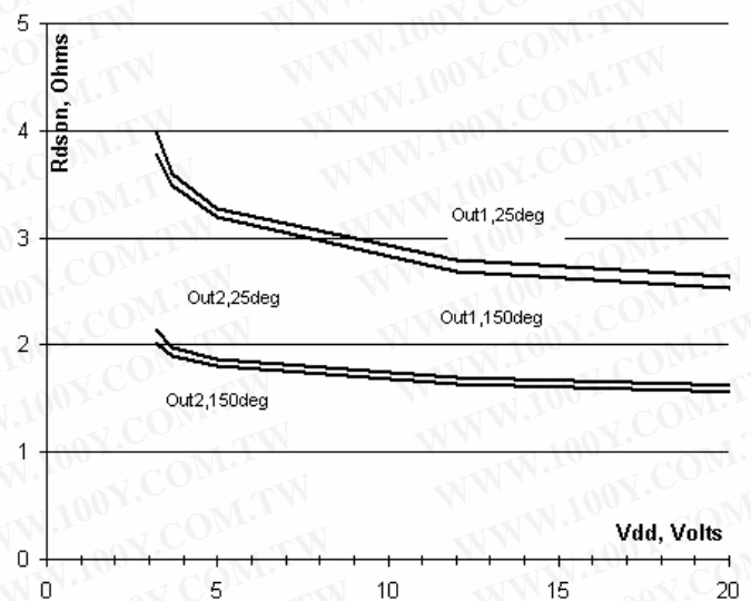
90245 Rdson vs. Voltage
