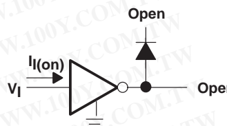
Figure 4. I_1 Test Circuit
