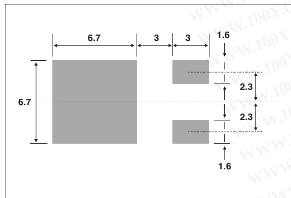
Figure 21: DPAK Foot Print Dimensions (in millimeters)
