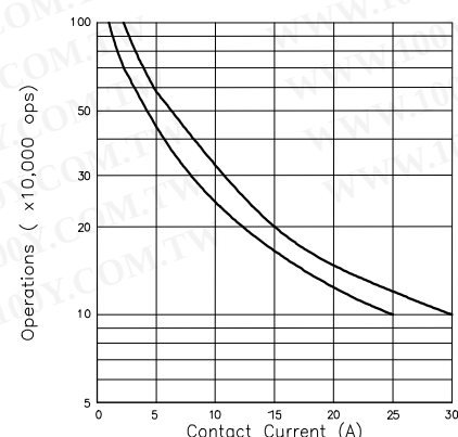
Life Curve
