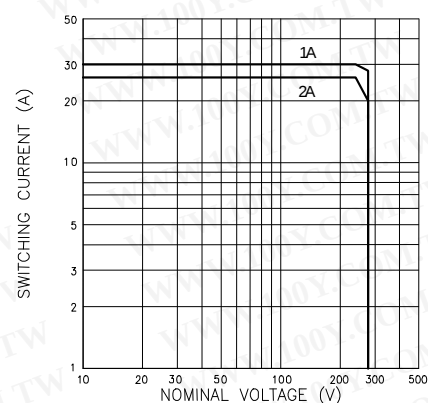
Contact Capacity
