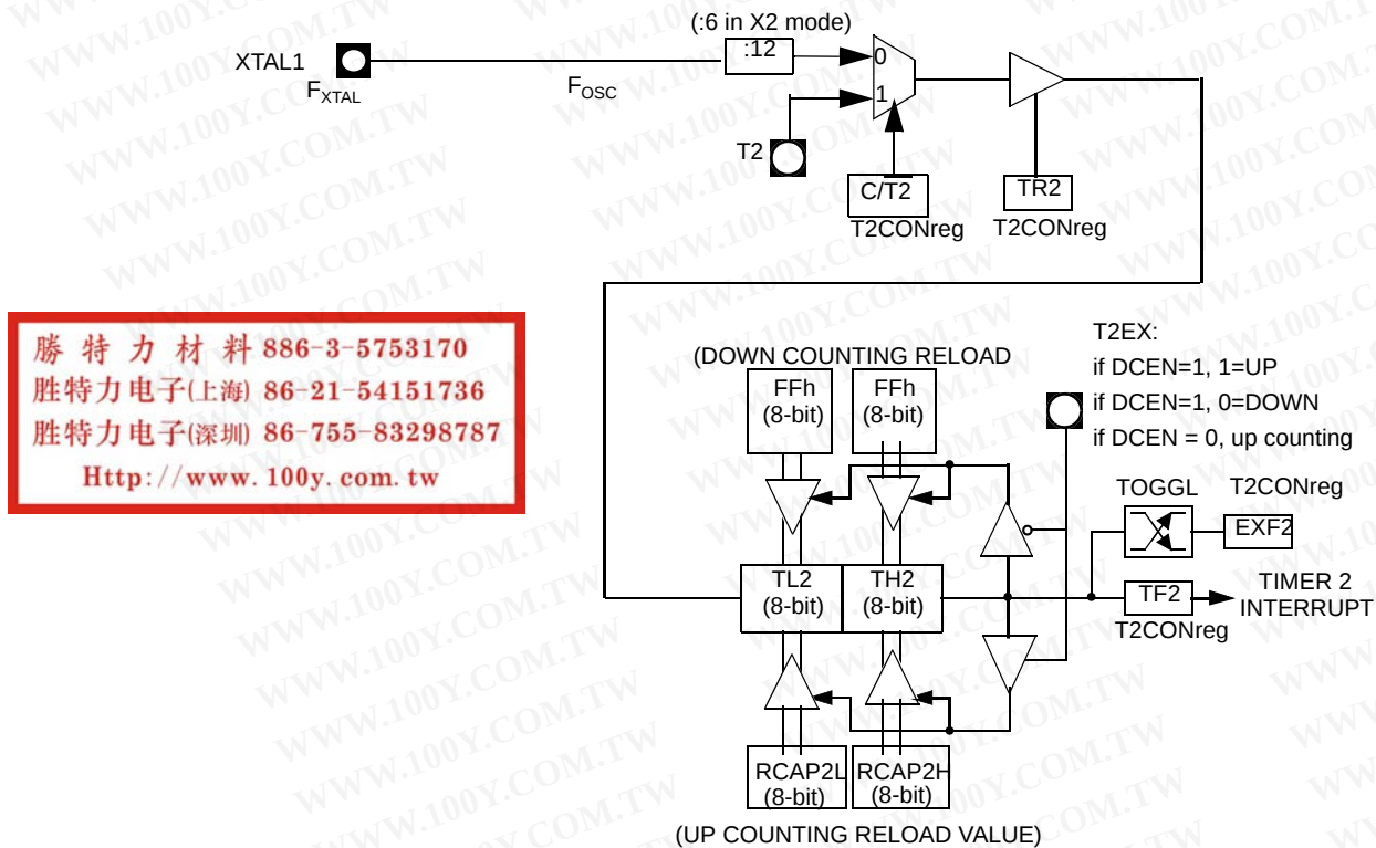
Figure 4. Auto-reload Mode Up/Down Counter (DCEN = 1)
