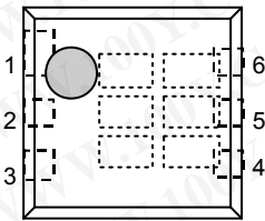
USP-6B (TOP VIEW)
