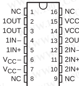
TLE2142 PW PACKAGE (TOP VIEW)
