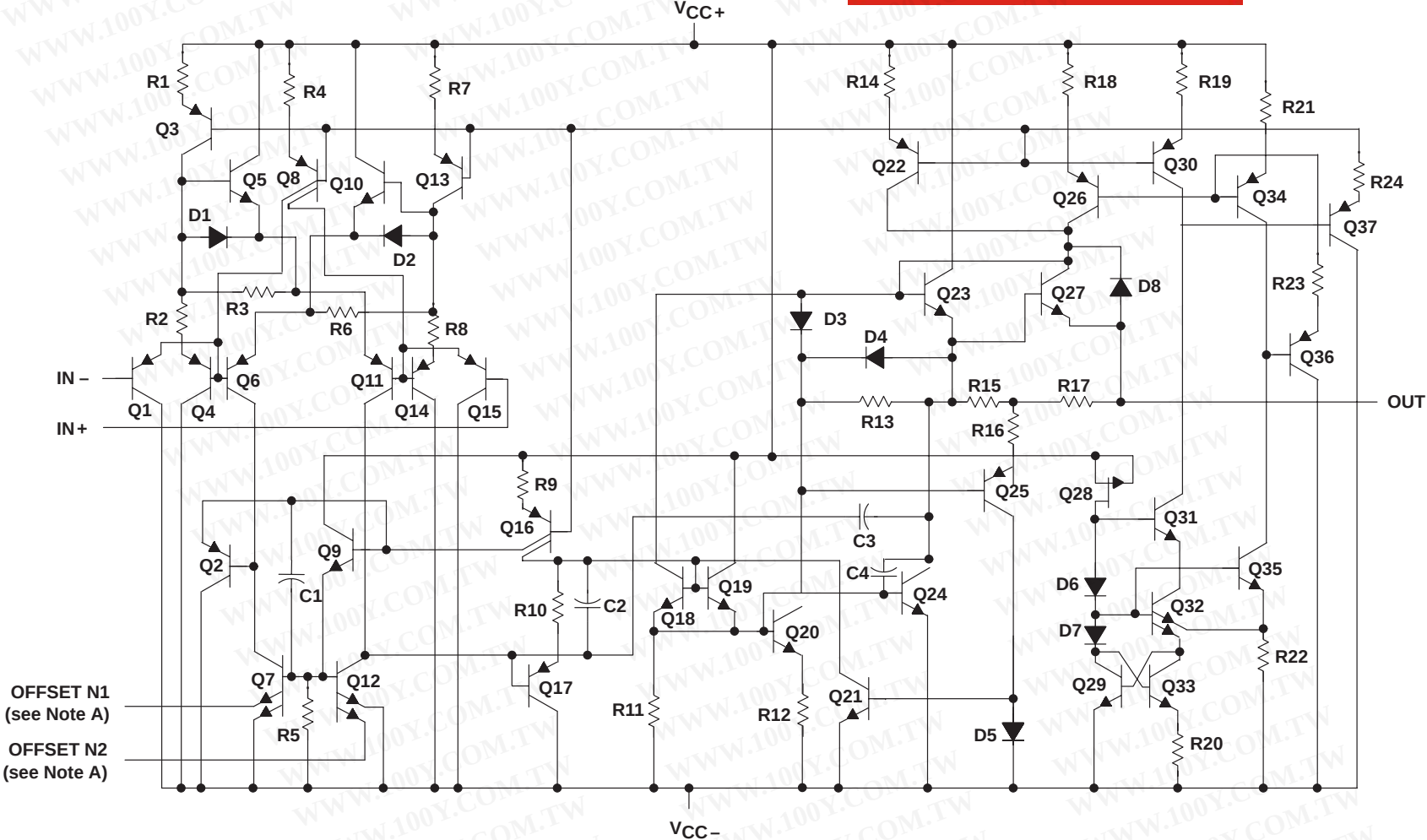
equivalent schematic
