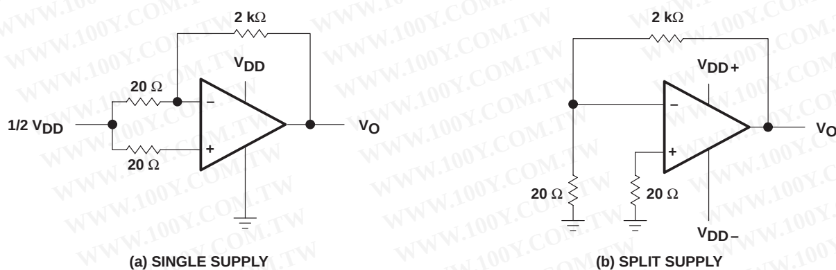
Figure 99. Noise-Test Circuit
