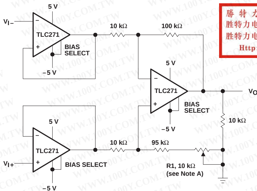
Figure 116. Low-Power Instrumentation Amplifier
