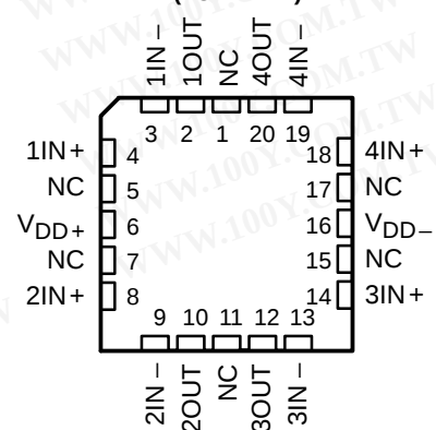
TLC2274 FK PACKAGE (TOP VIEW)
