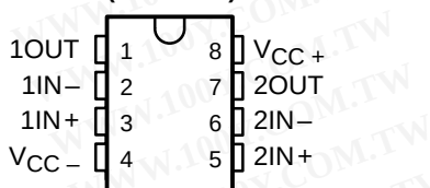
TL072, TL072A, TL072B D, JG, P, OR PW PACKAGE (TOP VIEW)
