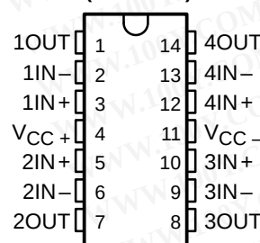
TL074, TL074A, TL074B D, J, N, OR PW PACKAGE TL074... W PACKAGE (TOP VIEW)
