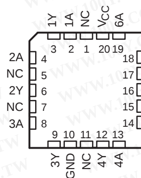
SN54LVU04A ... FK PACKAGE (TOP VIEW)
