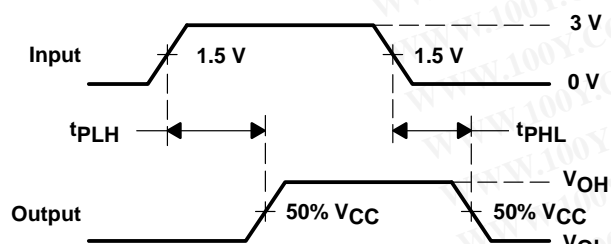
VOLTAGE WAVEFORMS
