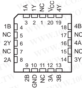
SN54HC02 . . . FK PACKAGE (TOP VIEW)
