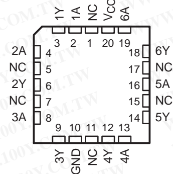
SN54AC04 . . . FK PACKAGE (TOP VIEW)
