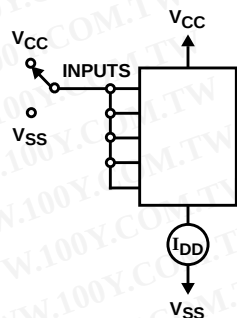
FIGURE 13. QUIESCENT DEVICE CURRENT TEST CIRCUIT
