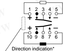
2-coil latching (Reset condition)
