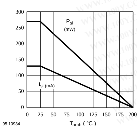
Figure 1. Derating diagram
