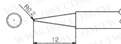
912-T2-LB Soldering Tip
