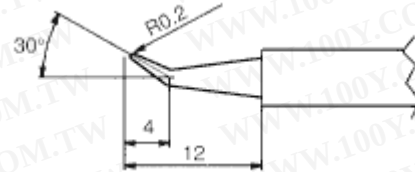
912-T2-02J Soldering Tip
