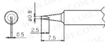
912-T2-08D Soldering Tip
