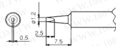
912-T2-12D Soldering Tip
