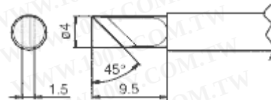
912-T2-K Soldering Tip
