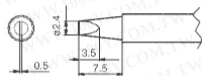
912-T2-24D Soldering Tip
