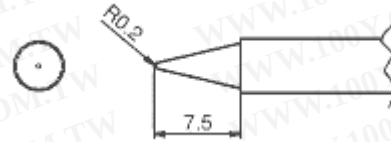
912-T2-B Soldering Tip
