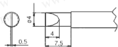
912-T2-4D Soldering Tip
