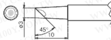
912-T2-3BCM Soldering Tip (Indent)
