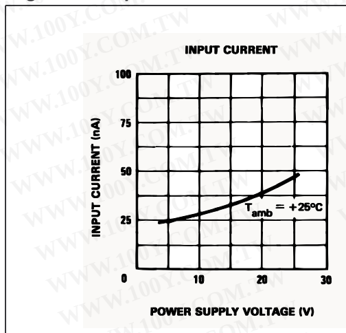
Figure 10. Input current
