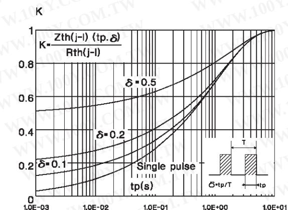
Fig. 3: Relative variation of thermal transient impedance junction to lead versus pulse duration.
