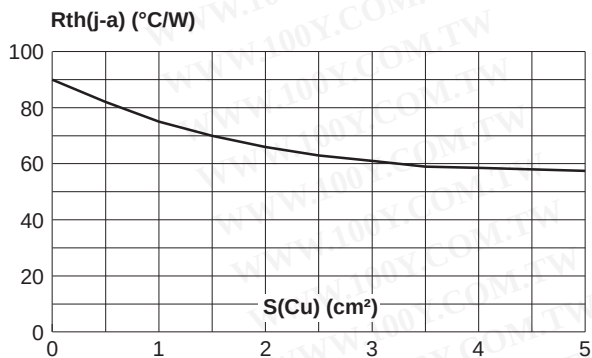
Fig. 8-2: Thermal resistance junction to ambient versus copper surface under each lead (Epoxy printed circuit board FR4, copper thickness: 35μm) (SMC).
