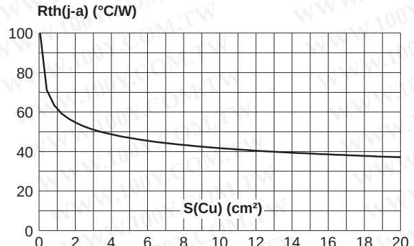
Fig. 8-3: Thermal resistance junction to ambient versus copper surface under each lead (Epoxy printed circuit board FR4, copper thickness: 35μm) (DPAK).
