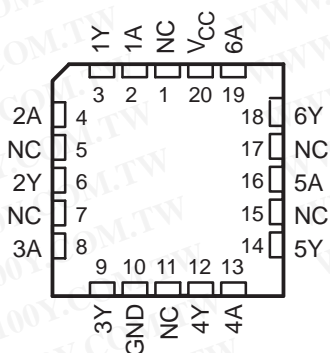
SN54ALS05A . . . FK PACKAGE (TOP VIEW)
