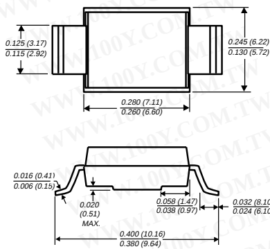
DO-215AA GULL WING
