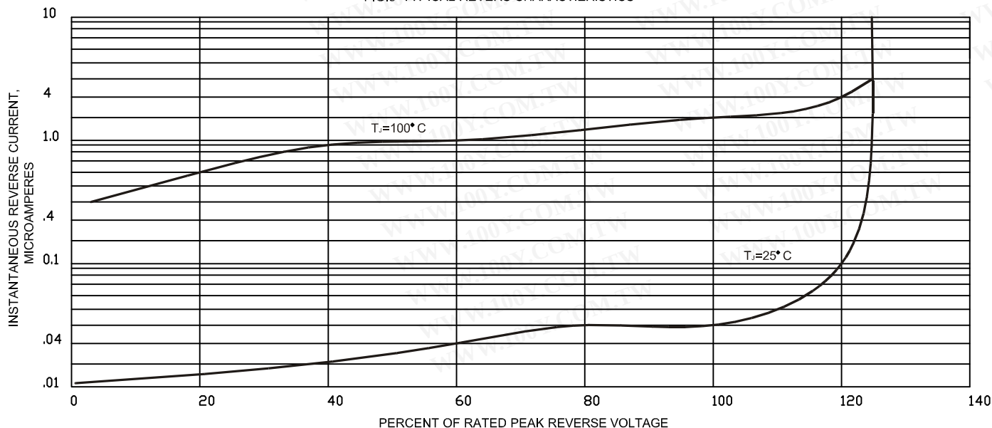
FIG.5- TYPICAL REVERS CHARACTERISTICS
