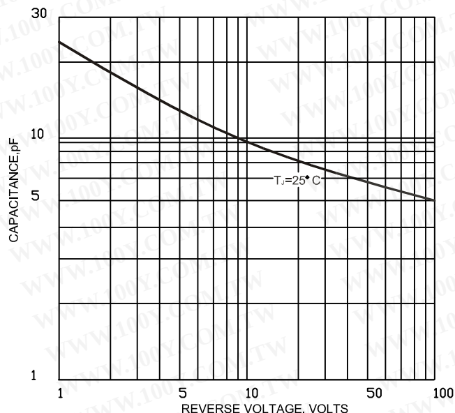
FIG.4-TYPICAL JUNCTION CAPACITANCE
