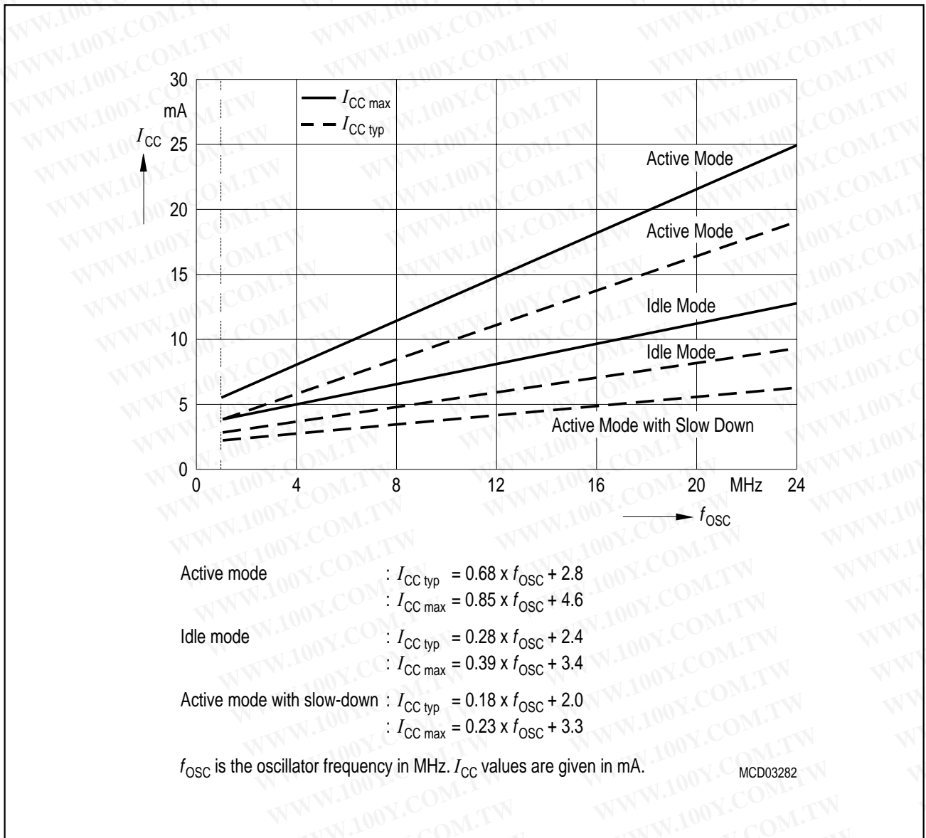
Figure 18 ICC Diagram
