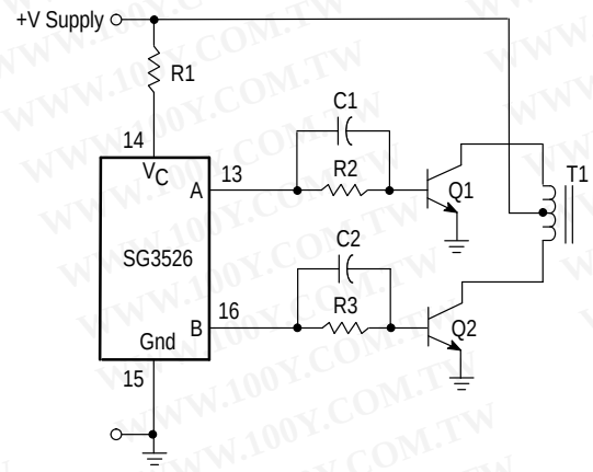
Figure 21. Push-Pull Configuration
