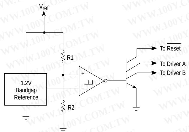
Figure 10. Undervoltage Lockout
