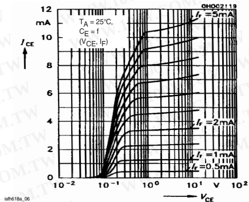
Fig. 9 Output Characteristics
