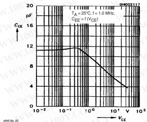
Fig. 8 Transistor Capacitance
