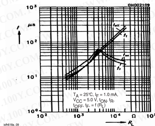
Fig. 11 Switching times (typ.)
