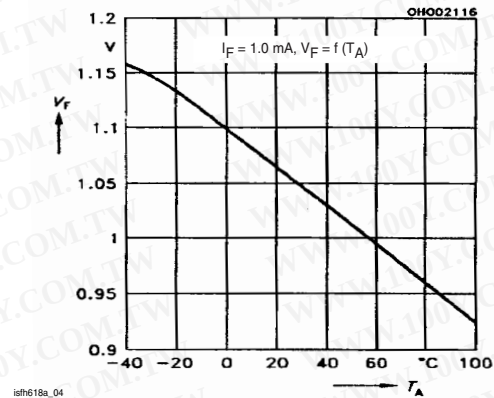
Fig. 7 Diode Forward Voltage (typ.)
