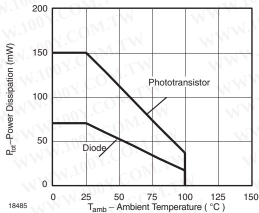
Fig. 1 Permissible Power Dissipation vs. Ambient Temperature
