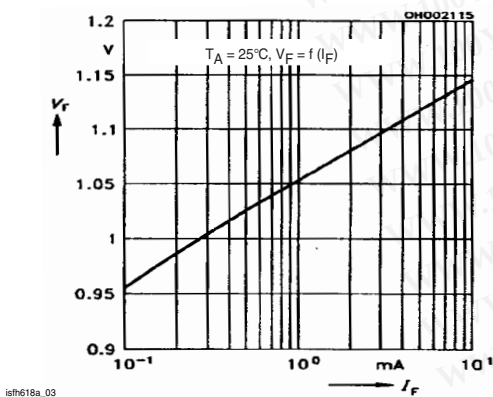
Fig. 6 Diode Forward Voltage (typ.)
