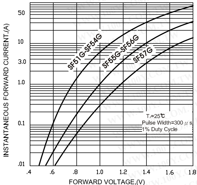
FIG.3-TYPICAL FORWARD CHARACTERISTICS
