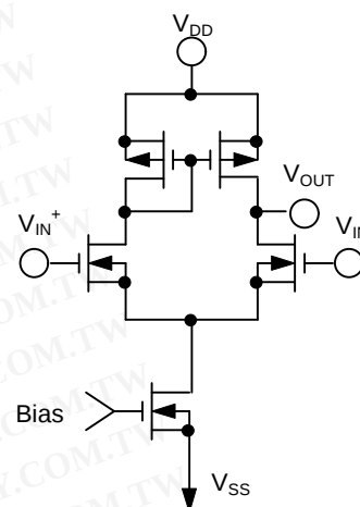
Figure 15 Comparator
