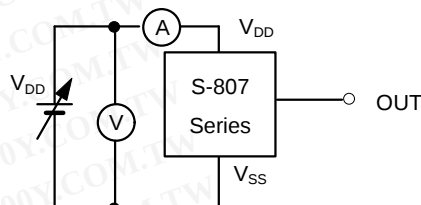
(2) Current consumption
