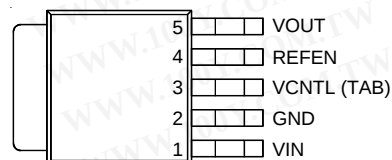
TO-252-5
