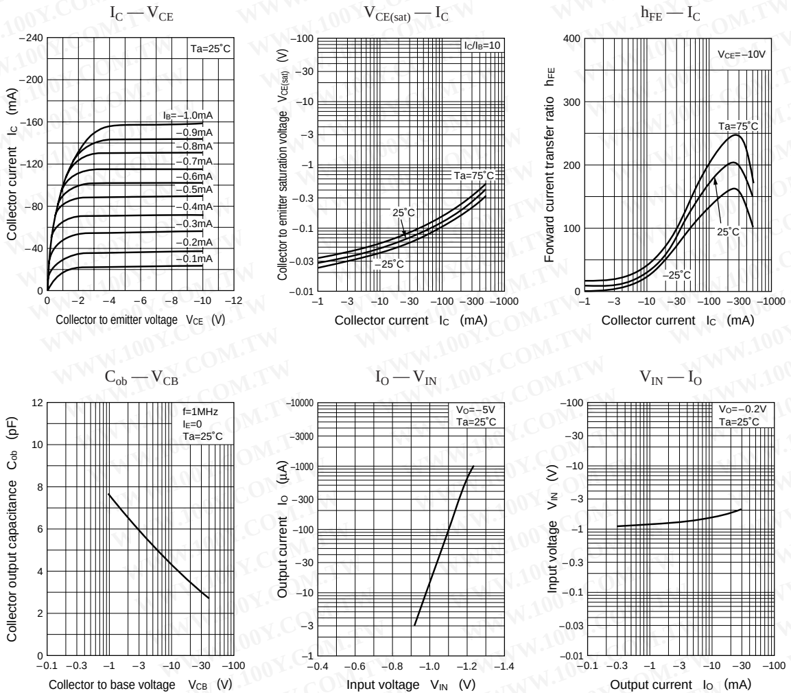
Characteristics charts of UN2122
