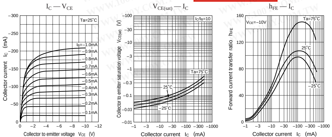
Characteristics charts of UN2122
