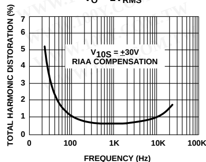
Distortion vs Frequency V_O = 1\text{V}_{\text{RMS}}
