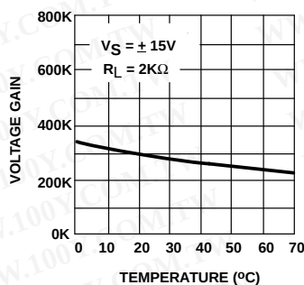
Open-Loop Gain as a Function of Temperature
