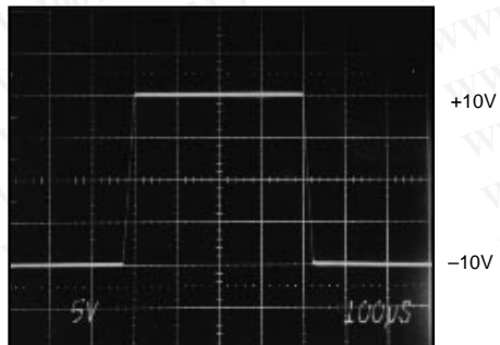
LARGE-SIGNAL RESPONSE, G = 10
