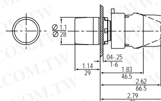
Round Illuminated Recessed Push Button
