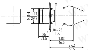
Square Mushroom-head Push Button
