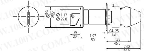
Round Plastic Emergency Stop Key-Reset
