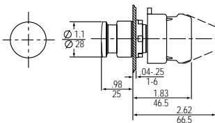
Round Metal Emergency Stop Twist-To-Reset (28 mm)
