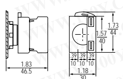
Single Contact Blocks With Quick Connect Terminals
