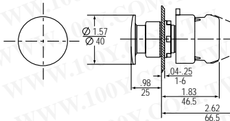
Round Metal Emergency Stop Twist-To-Reset (40 mm)
