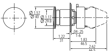
Round Push-Pull Mushroom-head Push Button
