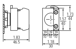
Single Contact Blocks With Screw Terminals
