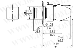
Square Illuminated Mushroom-head Push Button
