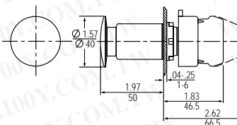
Round Plastic Emergency Stop Twist-To-Reset
