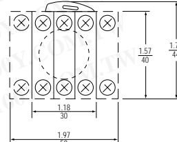
Typical Back Side View
