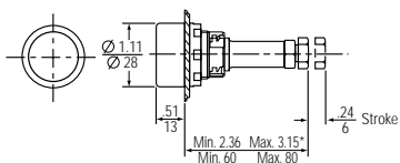
Round Reset Push Button
