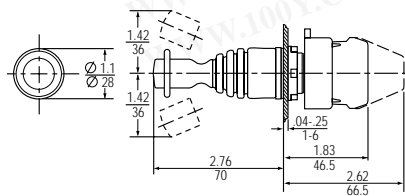
Round Joystick With Interlock
