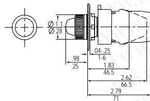
Round Indicating Light — Glass Lens
