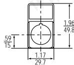
Square Standard Plate Holder
