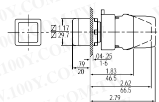
Square Illuminated Flush Push Button
