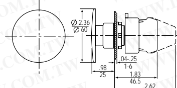
Round Mushroom-head Push Button (60 mm)
