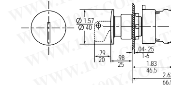
Round Metal Emergency Stop Key-Reset
