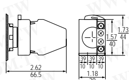
Double Contact Blocks With Screw Terminals
