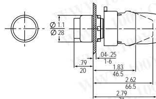
Round Illuminated Extended Push Button
