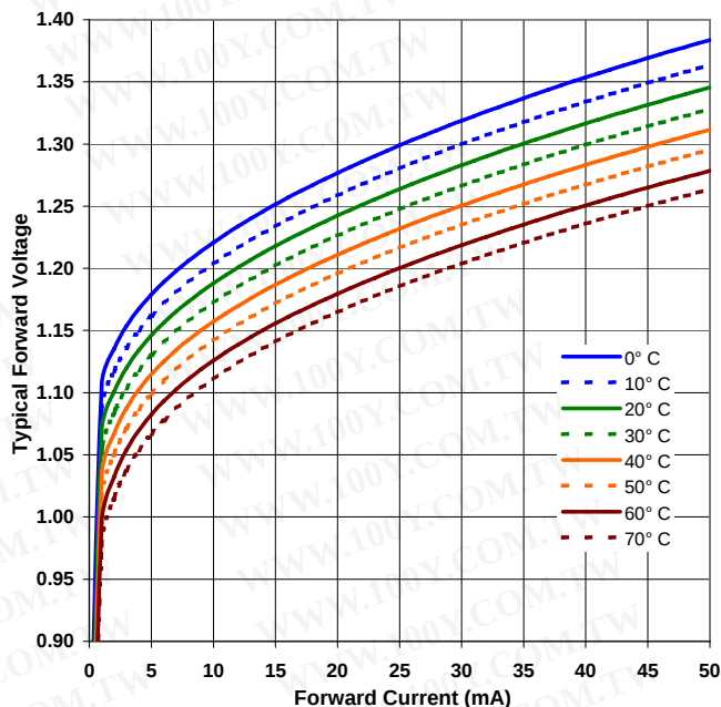
OPB710 - Forward Voltage vs Forward Current vs Temp
