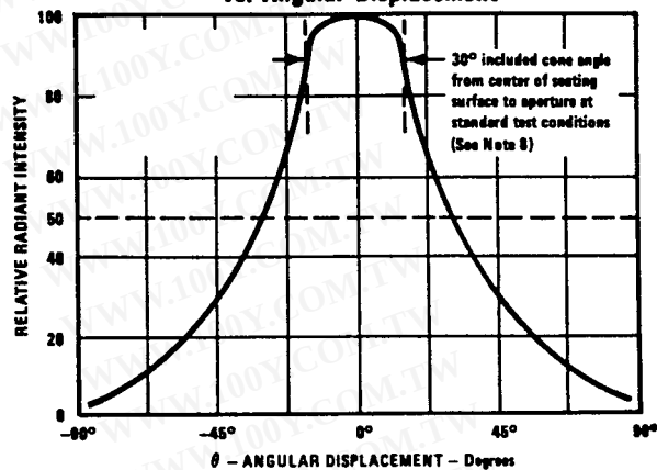
OP293 — Relative Radiant Intensity vs. Angular Displacement
