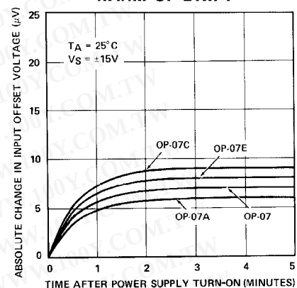
WARM-UP DRIFT
