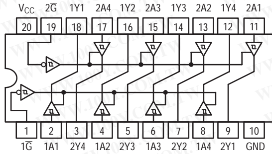
SN74LS244
