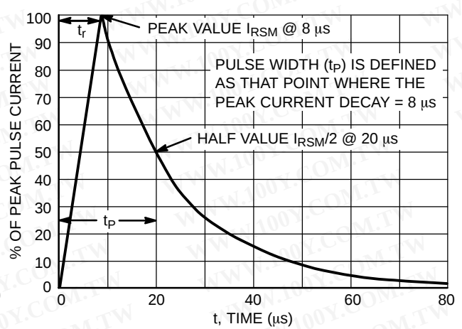
Figure 4. 8 \times 20 \mu\text{s} Pulse Waveform
