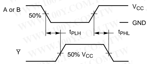
Figure 3. Switching Waveform
