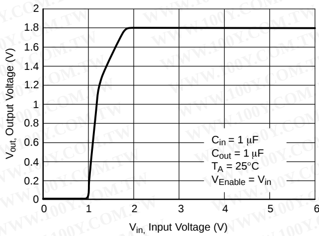
Figure 24. Output Voltage vs. Input Voltage
