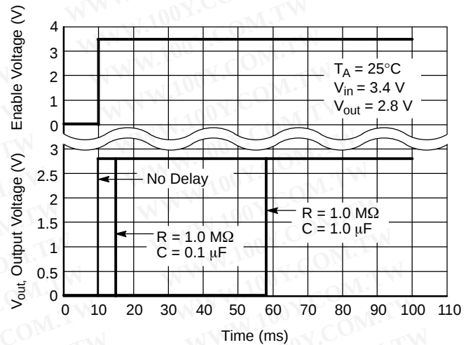
Figure 33. Delayed Turn-on
