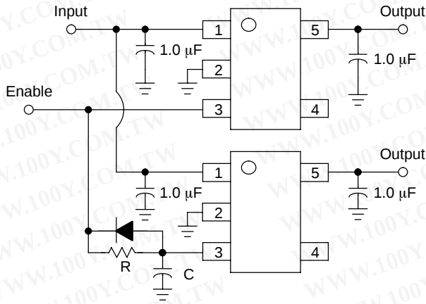
Figure 32. Delayed Turn-on
