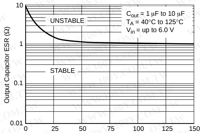
Figure 29. Stability
