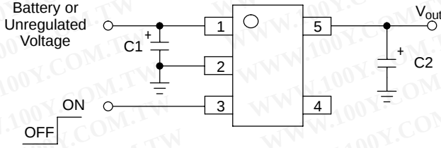
Figure 27. Typical Application Circuit
