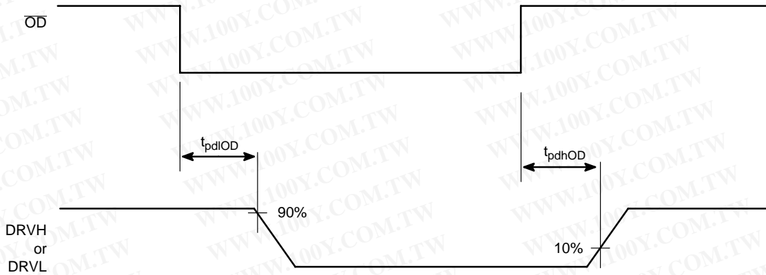
Figure 2. Output Disable Timing Diagram
