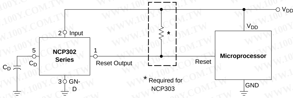
Figure 38. Microprocessor Reset Circuit
