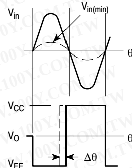
Figure 10. Zero Crossing Detector (Split Supplies)
